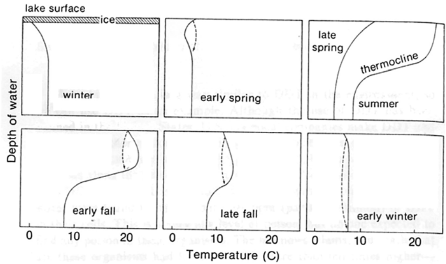
Figure 11-5. Seasonal cycle of temperature patterns in a typical temperate-zone lake. Overturn is indicated by dashed lines and it is much more extensive in the fall than in the spring. The thermocline might develop typically at depths of 5 to 25 meters, depending on the depth and turbidity of the lake and the wind pattern of the area.
