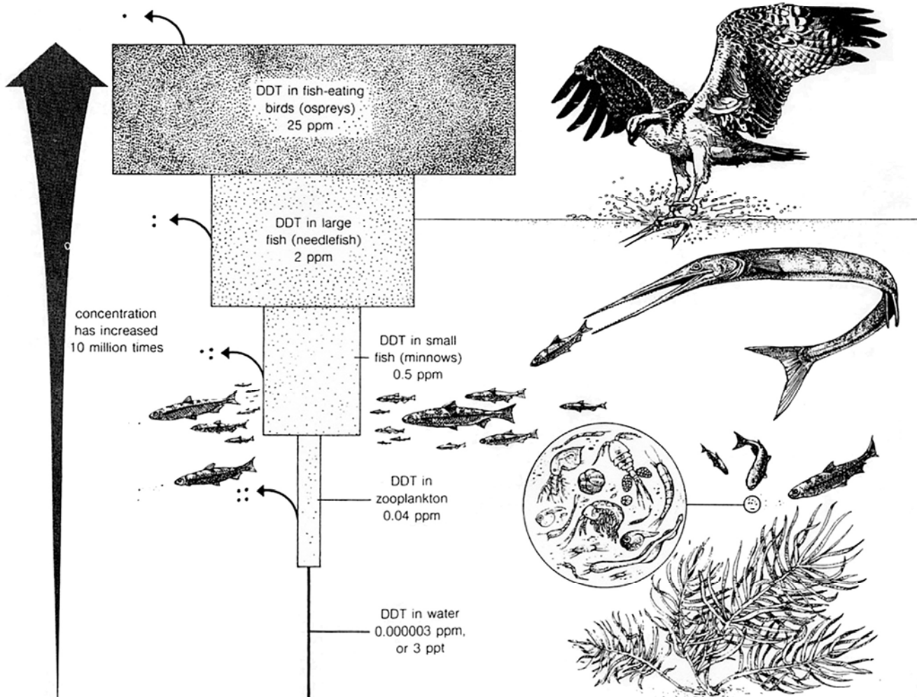
Figure 3.18 As DDT is passed from organism to organism in the Long Island Sound food chain, the concentration is magnified about 10 million times. Dots represent DDT, and arrows show small amounts lost in the daily activities of the organisms.
